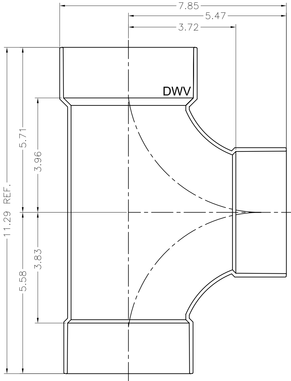
SDR 35 2 WAY CLEANOUT WITH DWV HUB DWV X SEWER X SEWER 4X4X4
